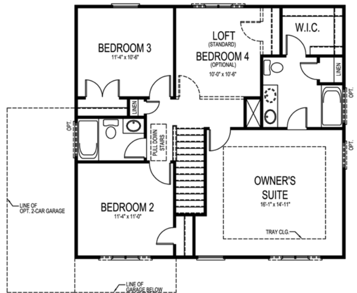
SECOND FLOOR
